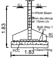
SECTION OF FOOTING
