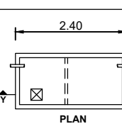
FOUNDATION DETAILS
