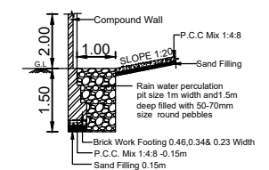
RAINWATER HARVESTING TRENCH
