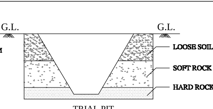
TRIAL PIT
