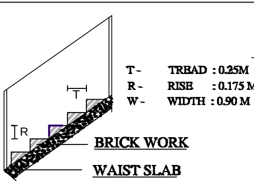
STAIRCASE & ENTRANCE STEPS
