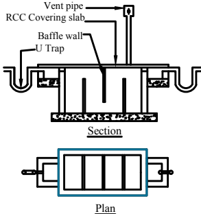
Septic Tank With U Trap
