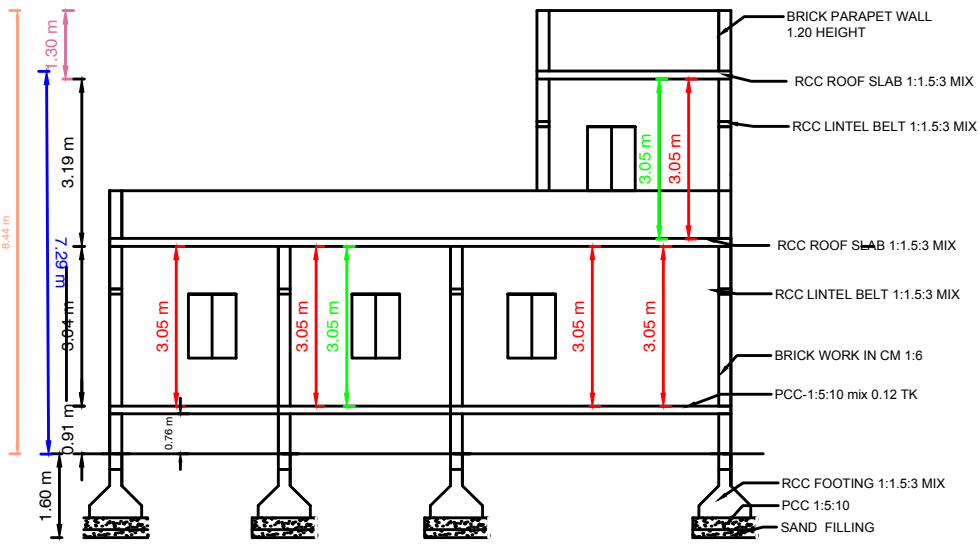
SECTION "AB"
