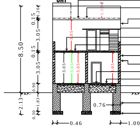
SECTION ON "XY"
