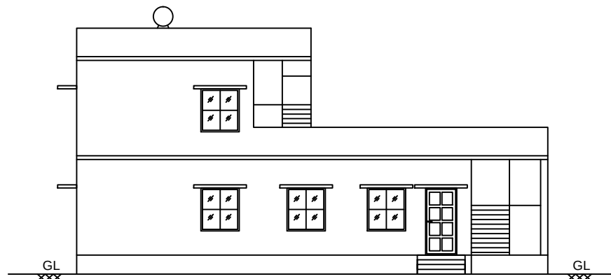
ELEVATION - EAST FACING
