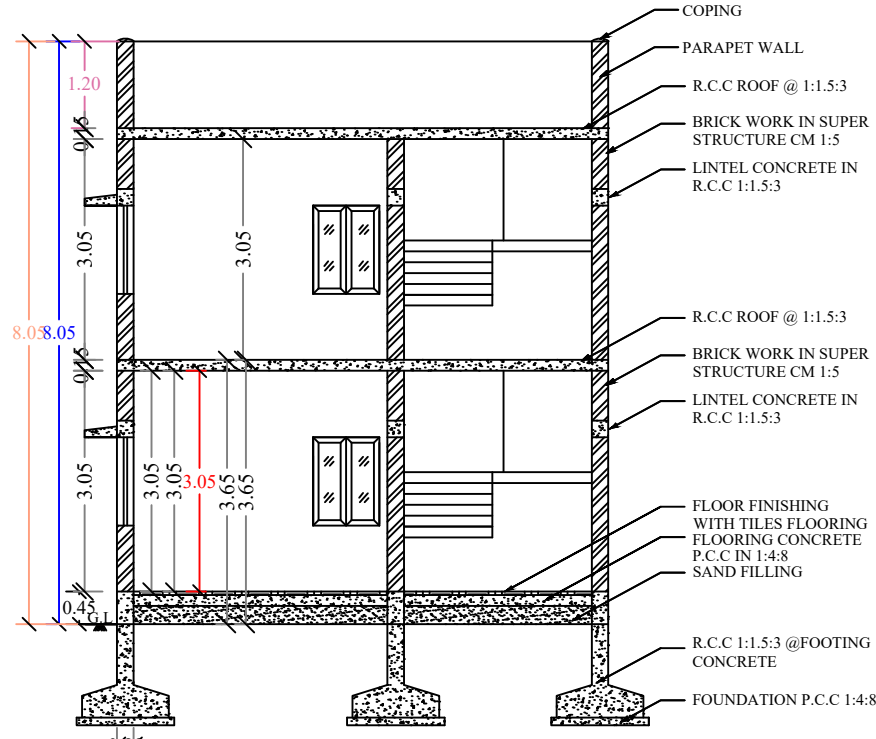
SECTION-AB
