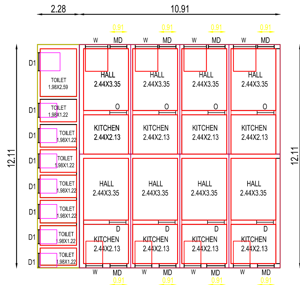
GROUND FLOOR PLAN (100)
