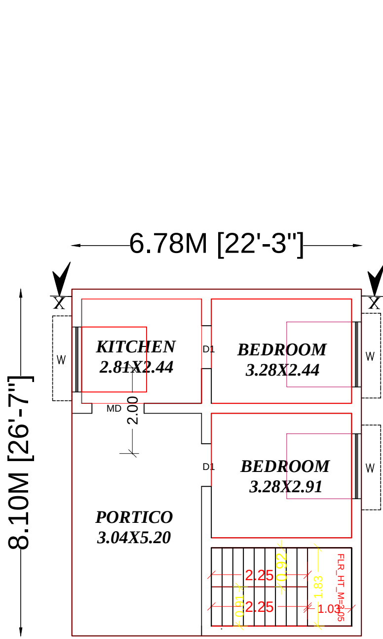
PLAN
