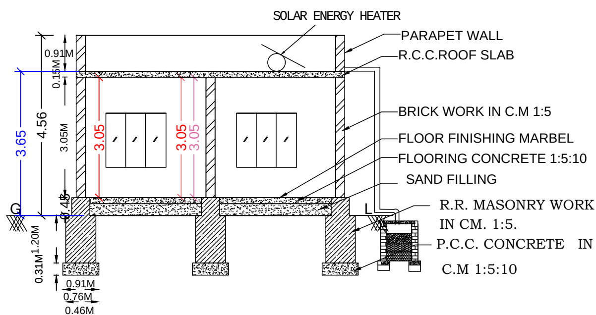
SECTION - XX
