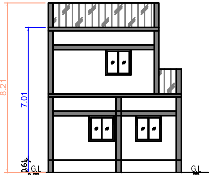
ELEVATION (SOUTH SIDE VIEW)
