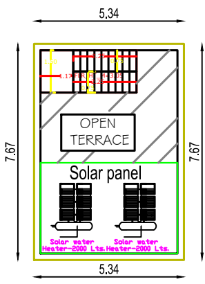
TERRACE FLOOR PLAN (Scale 1:100)
