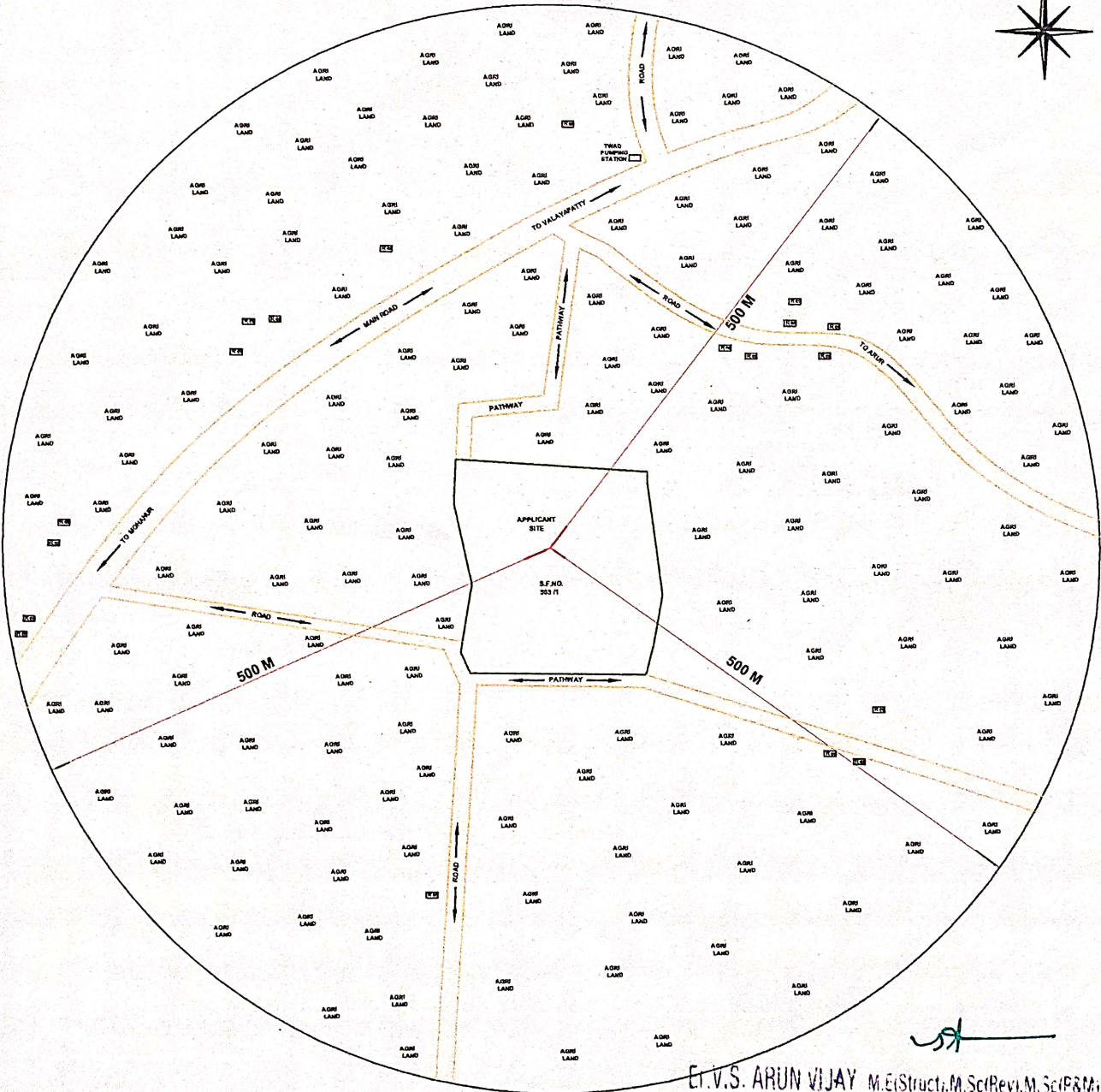
TOPO PLAN
