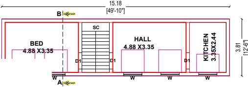
PROPOSED FIRST FLOOR PLAN
