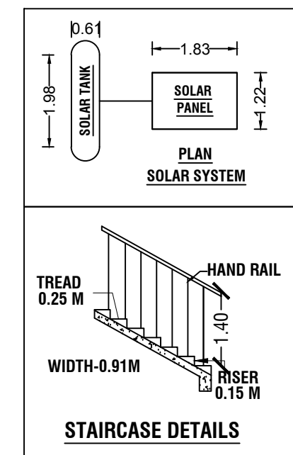
STAIRCASE DETAILS
