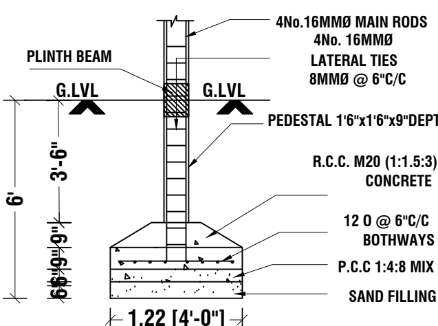
FOUNDATION DETAIL [SCALE: 1:50]
