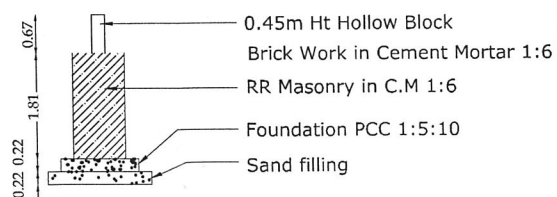
FOUNDATION DETAILS
