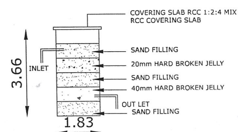
WASTE WATER RECYCLE UNIT
