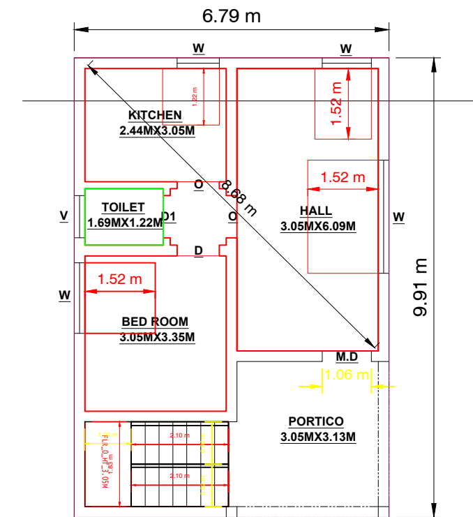
G.F. PLAN
