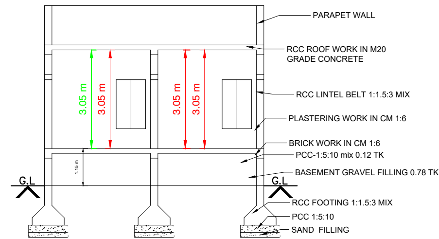
SECTION"AB"
