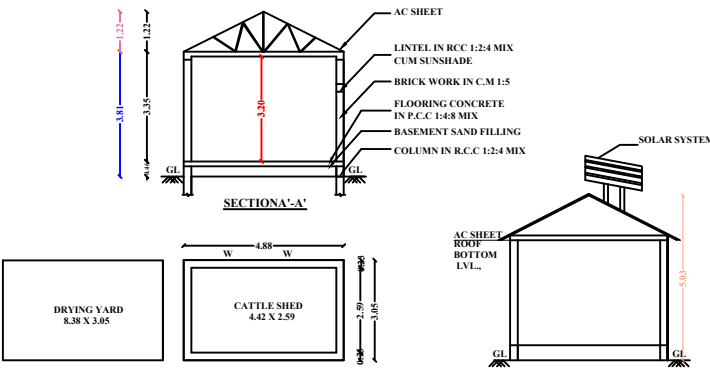
CATTLE SHED -PLAN
