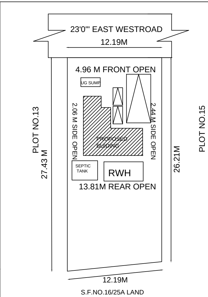
SITE PLAN SCALE :1:250
