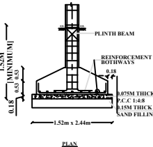
TYP.DET. COLUMN FOOTING
