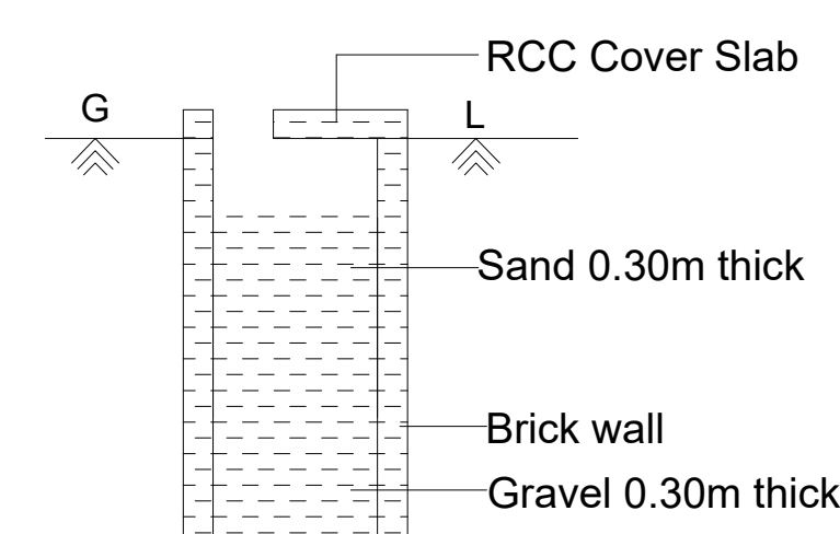
Organic Filter Details (Not to Scale)
