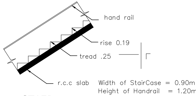
STAIR
