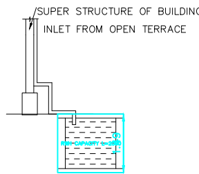
RAINWATER HARVESTING
