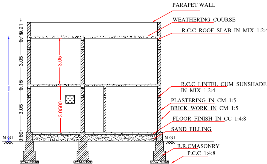
SECTION ON-"AB"
