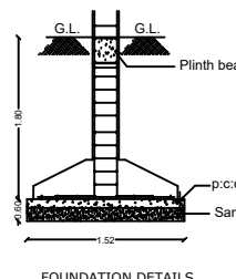
FOUNDATION DETAILS
