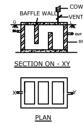
SEPTICTANK DETAILS
