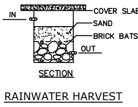
RAINWATER HARVEST
