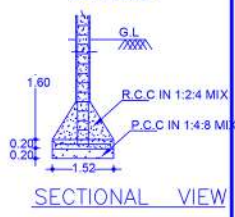
JMN DETAILS
