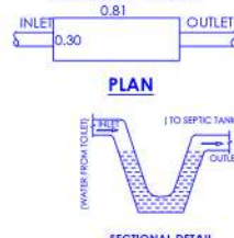
SECTIONAL DETAIL
