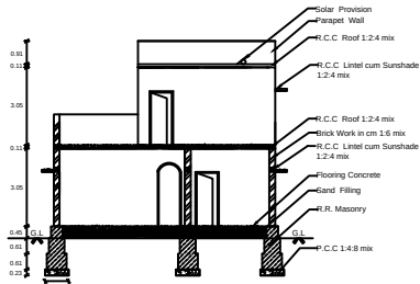
SECTION ON "ABC"
