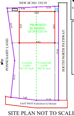
SITE PLAN NOT TO SCALE
