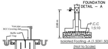
SECTION " AB "
