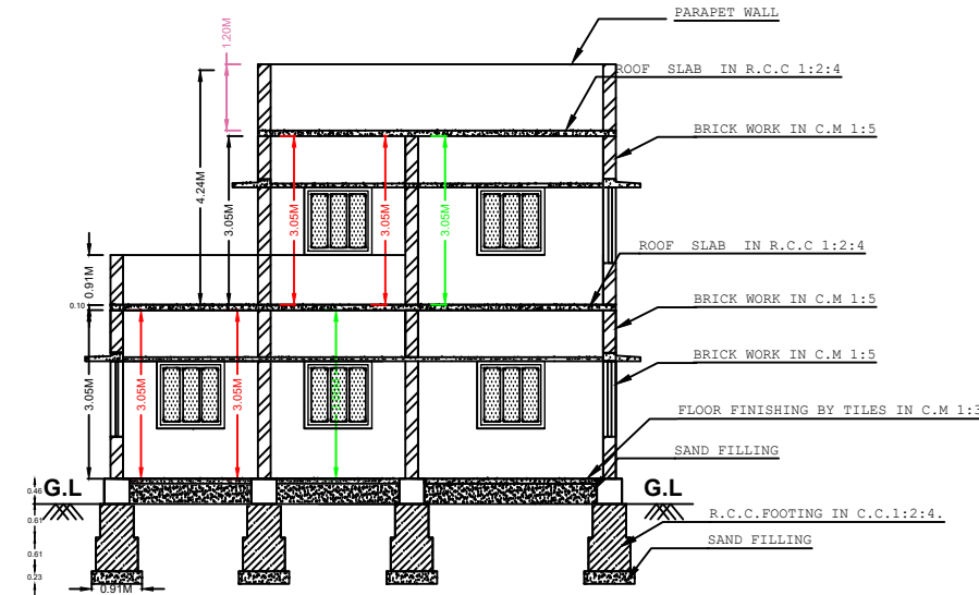
SECTION ON -XY
