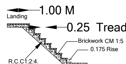
Staircase Details.
