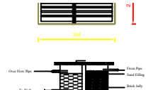
WATER TANK _2000 LITER
