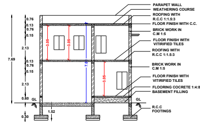
SECTION ON "S S"
