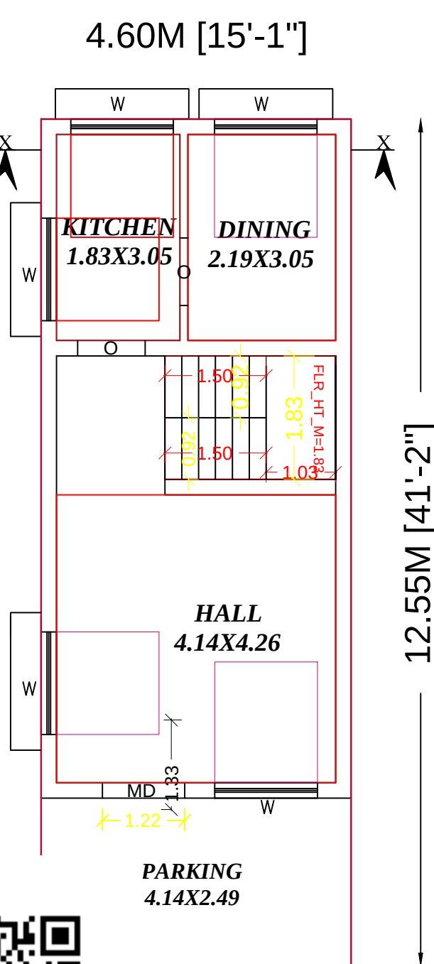
FLOOR PLAN
