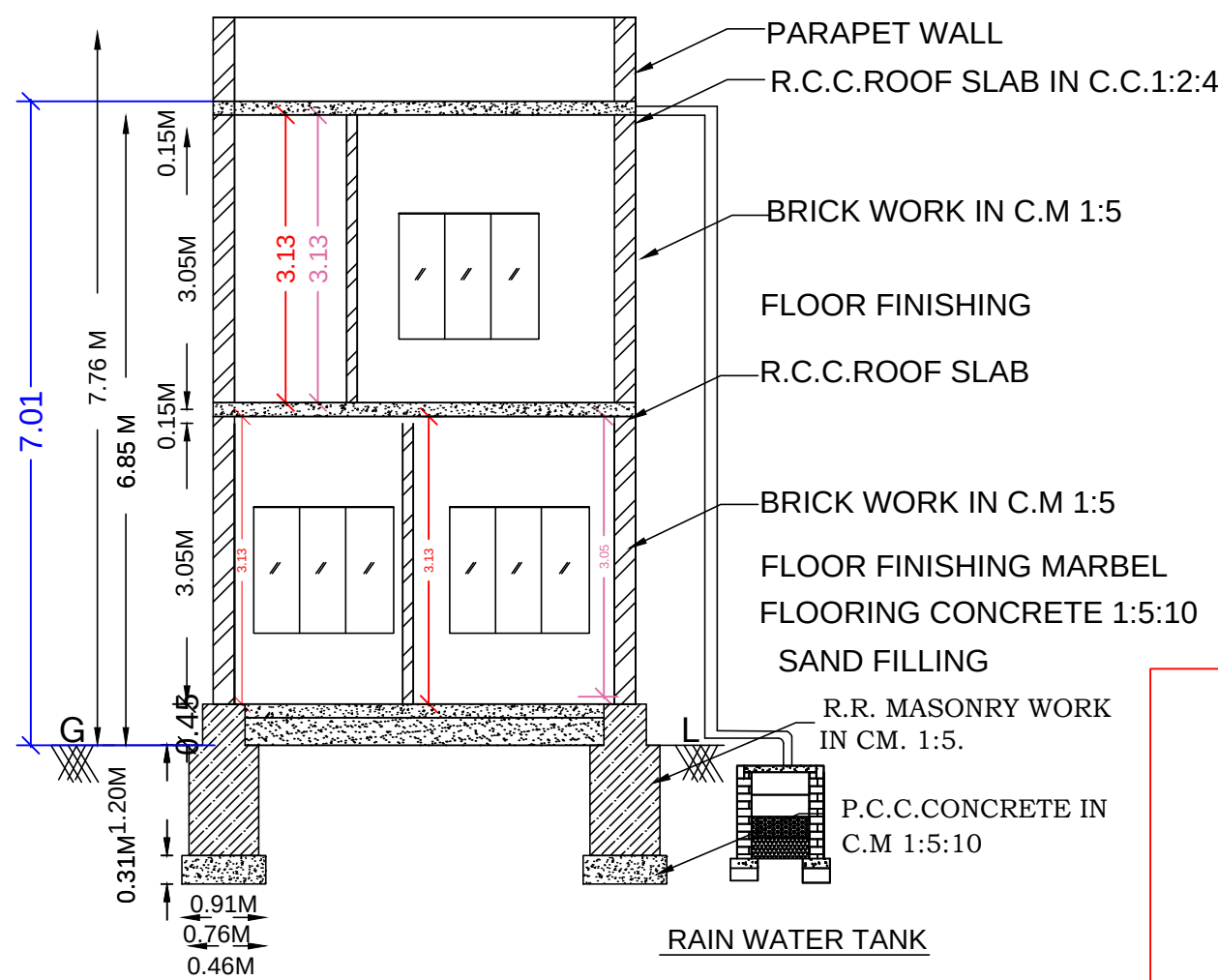
SECTION - XX
