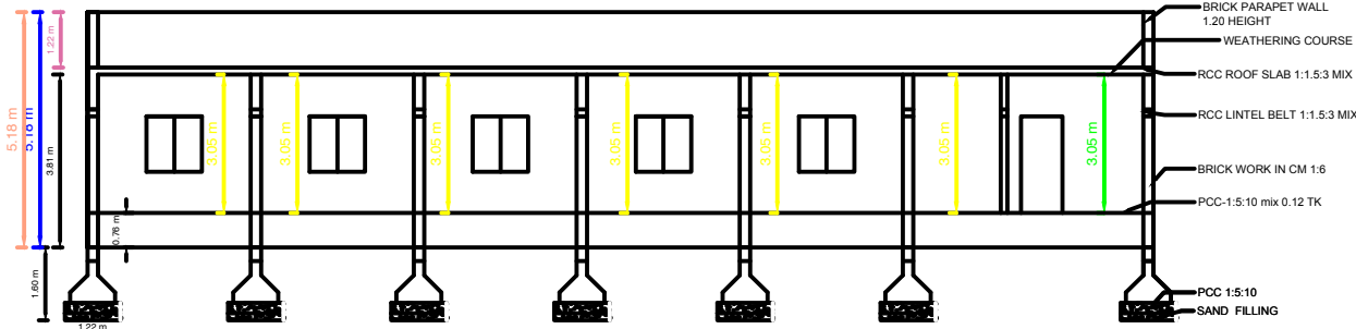
SECTION " AB "
