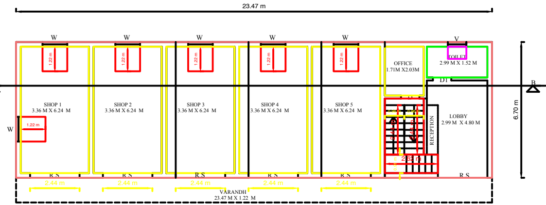
COMMERCIAL - PLAN
