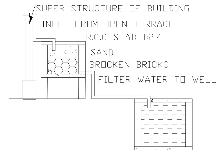
RAINWATER HARVESTING
