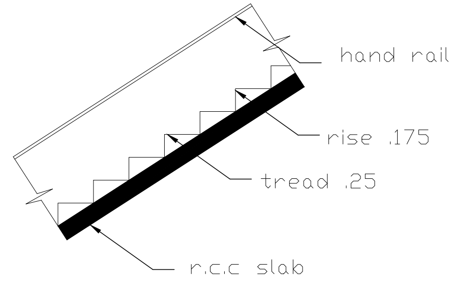
STAIR
