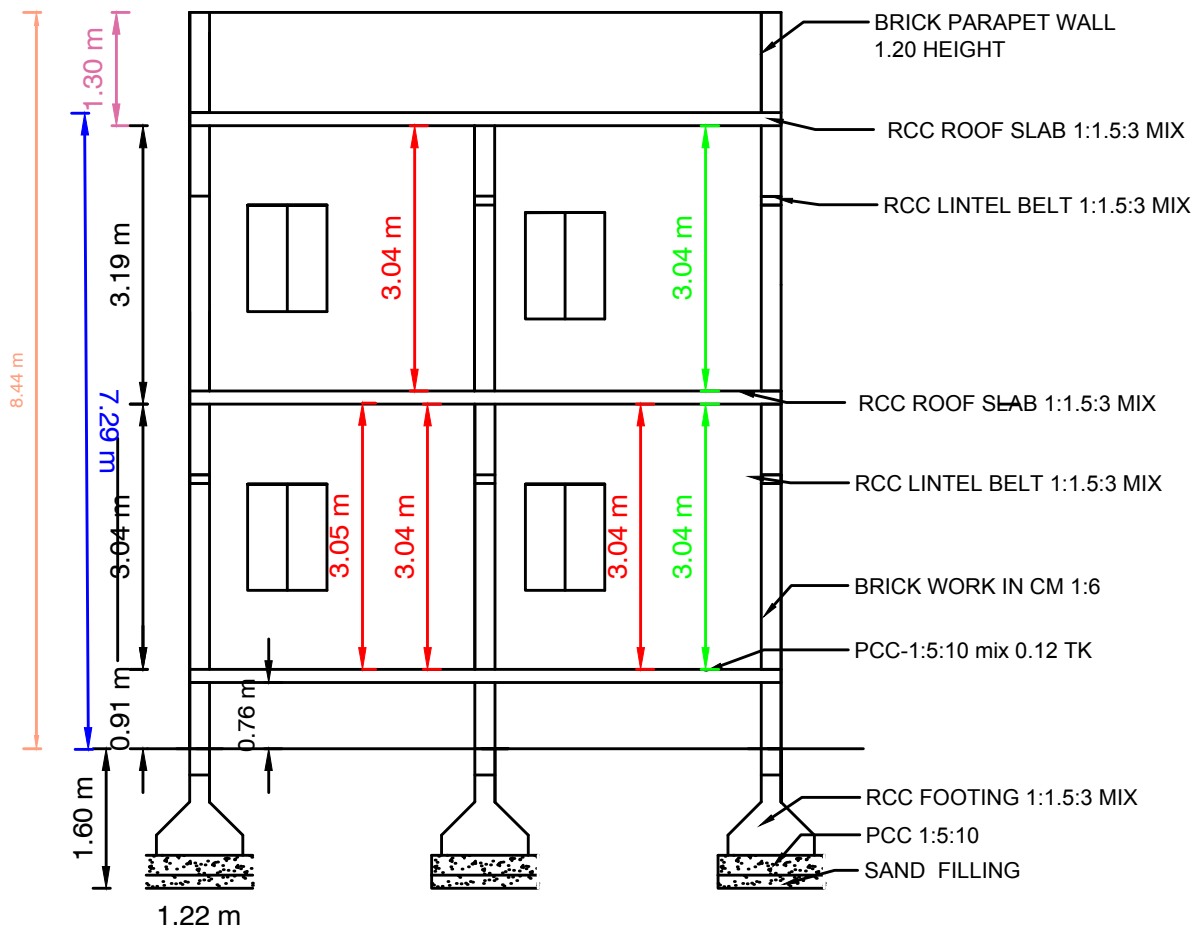
SECTION "AB"
