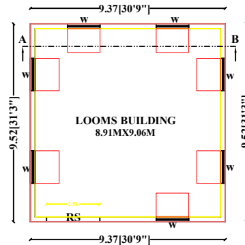
LOOMS BUILDING - PLAN
