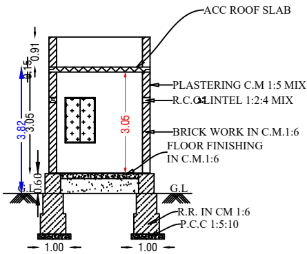
SECTION ON-"AB"
