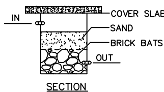
RAINWATER HARVEST
