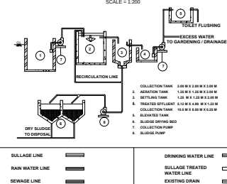
SECTIONAL ELEVATION FOR SEWAGE / SULLAGE TREATMENT PLANT NOT TO SCALE: SCALE = 1:200
