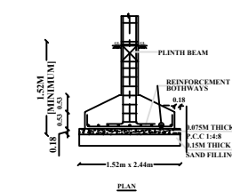
TYP.DET. COLUMN FOOTING
