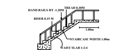
STAIRCASE DETAILS
