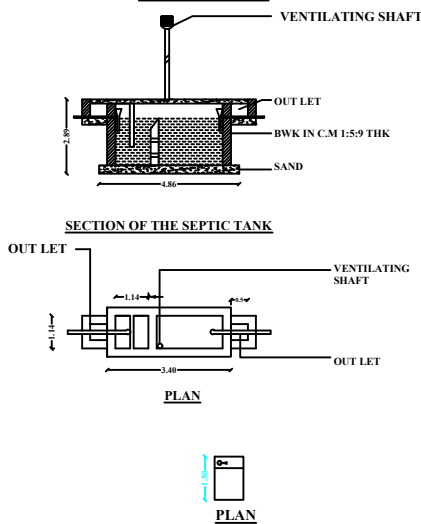
SEPTIC TANK
