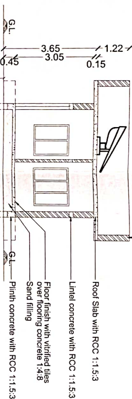
SECTION "AB"
