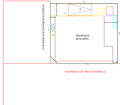
SITE PLAN
