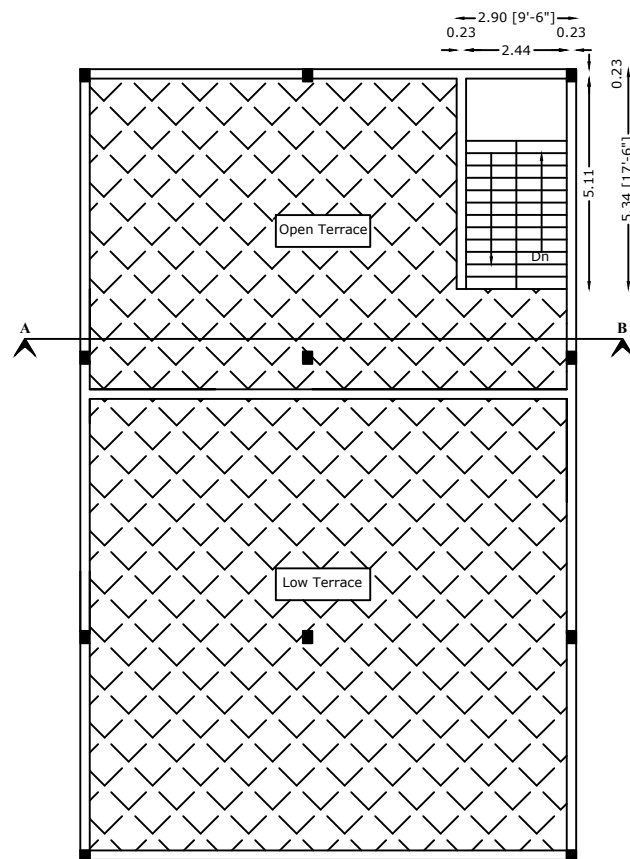
ROOF FLOOR PLAN SCALE - 1:100
