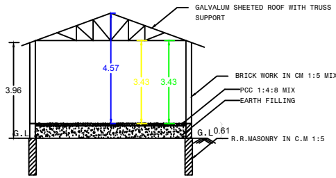
CROSS SECTION ON 'AA'
