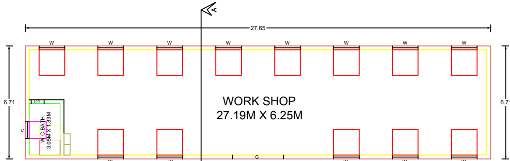
PROPOSED PLAN
