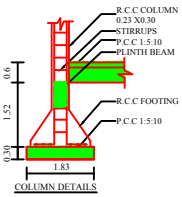
COLUMN DETAILS
