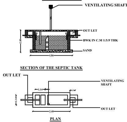
SEPTIC TANK
