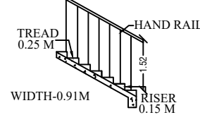
STAIRCASE DETAILS
