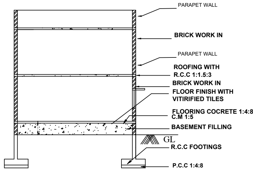
SECETION
