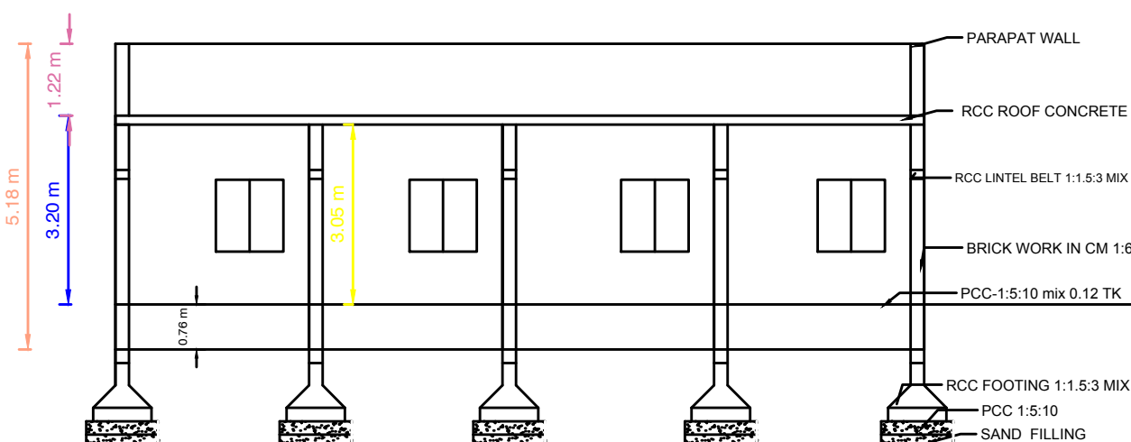
SECTION"AB"
