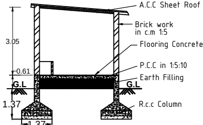
A.C.C Shed Section
