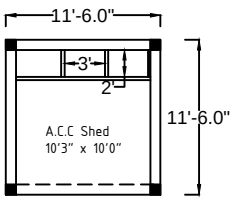
A.C.C Shed Plan (Cattle Shed)
