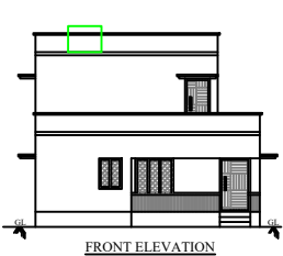
FRONT ELEVATION
