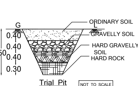
Trial Pit
