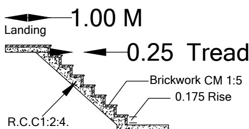
Staircase Details.
