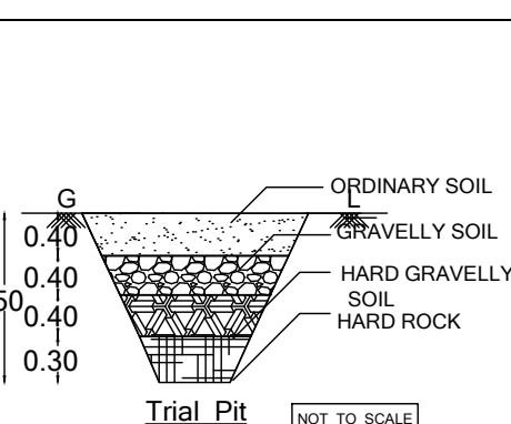
Trial Pit
