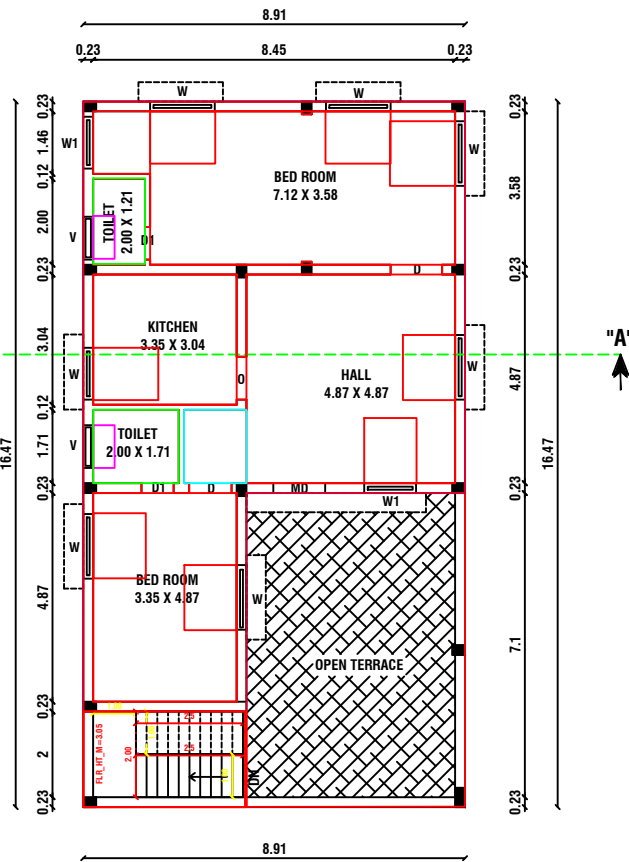
FLOOR - FIRST & TERRACE PRO. FIRST & TERRACE FLOOR PLAN
