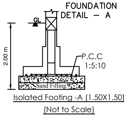
FOUNDATION DETAIL - A
