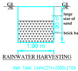
SECTION " AB "
