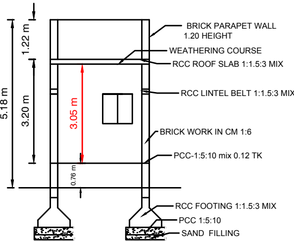
SECTION " AB "
