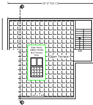
ROOF FLOOR PLAN SCALE-1:100
