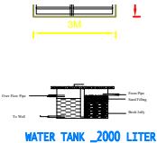
WATER TANK _2000 LITER
